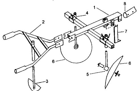
Figure 1: Components of the disc ridger 1: beam with draw bar attachment; 2: handle; 3: tie-maker; 4: attachments for distance between discs and disc angle; 5: king pins with disc shafts; 6: discs; 7: duckfoot-tine; 8: draw bar
